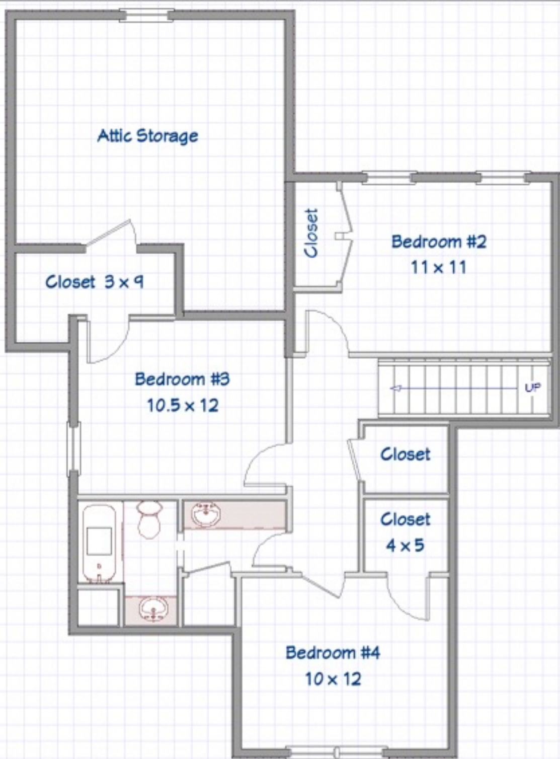
10 Butternut Court Upstairs Floor Plan
